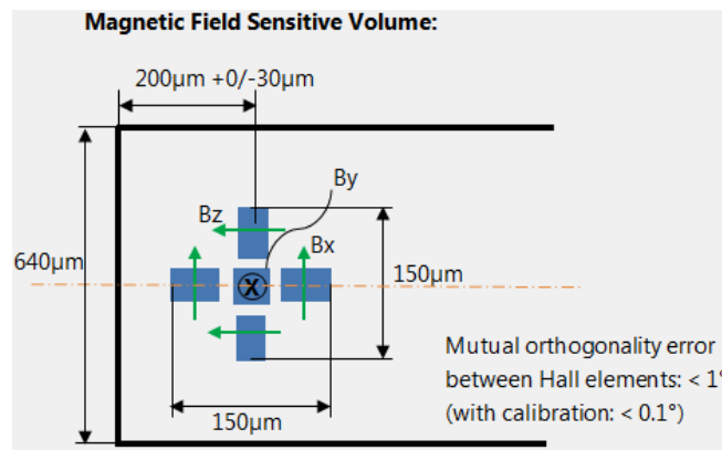
Figure 3. Overall magnetic field sensitive volume (MFSV) of the applied fully integrated 3D Hall sensor
